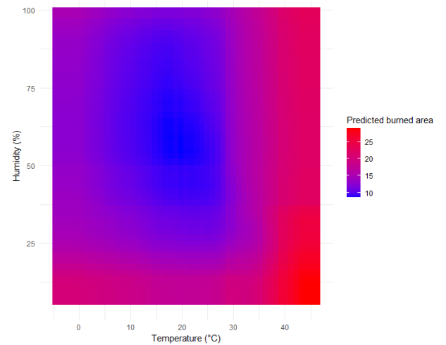
Figure 15: PDP for Temperature and Humidity
