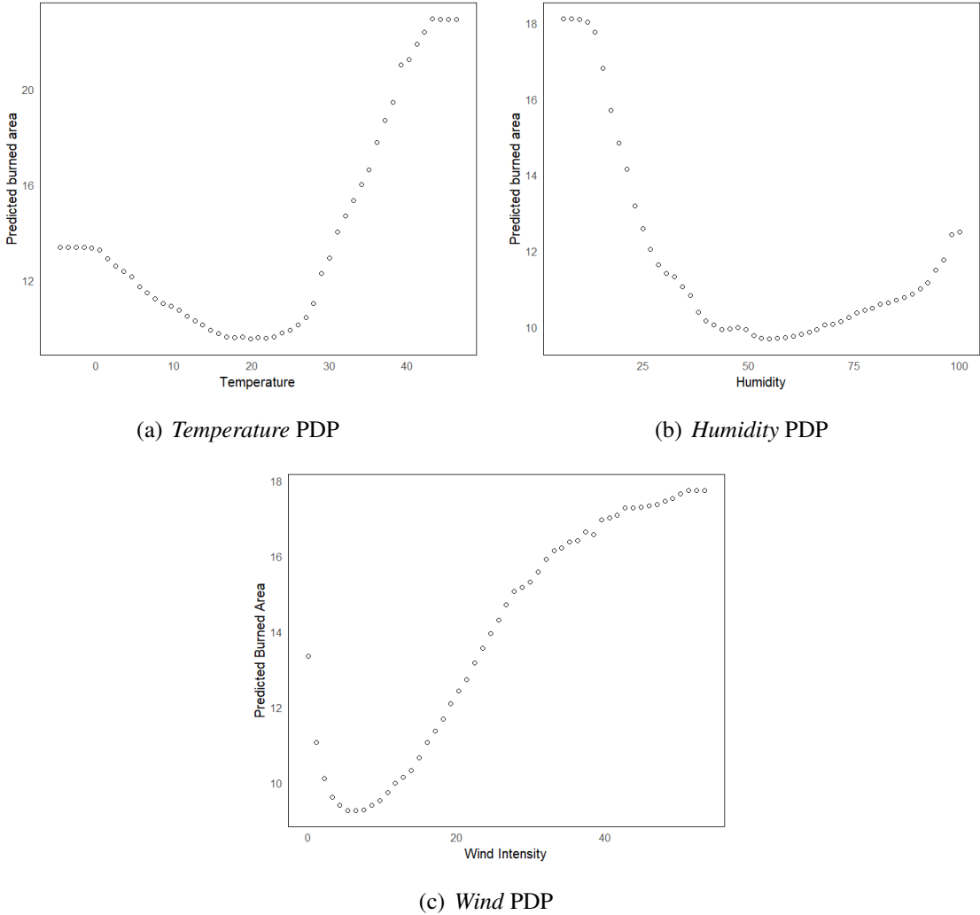
Figure 14: Severity PDPs
