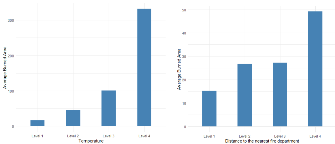
(a) Average burned area per ignition vs Temperature
